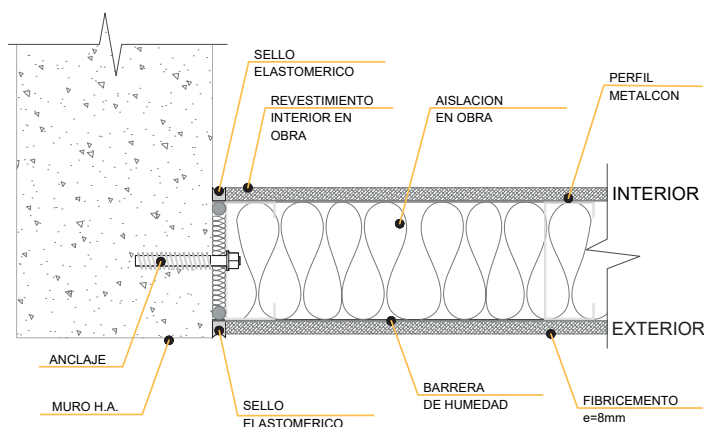
CORTE VISTA LATERAL ANTEPECHO PREF.
